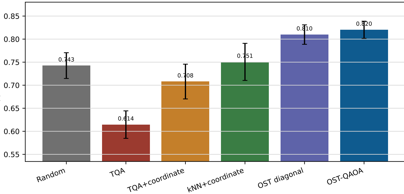
mean approximation ratio
