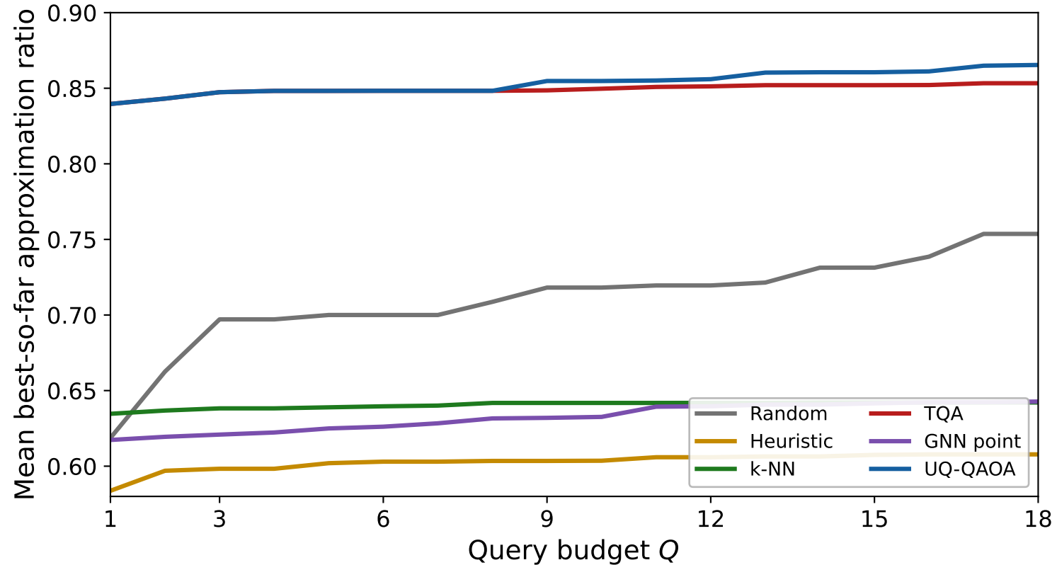
Best-so-far ratio vs. query budget -- n = 14, p = 3
