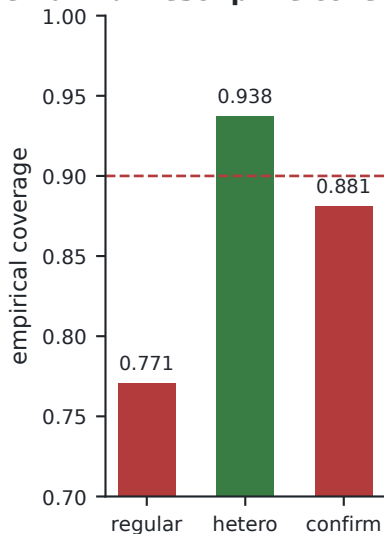
b Descriptive coverage gate
