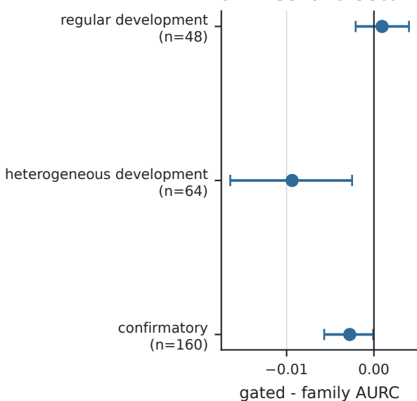
a Effect and 95% interval
