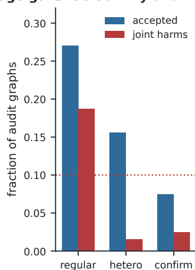
c Selectivity and harm
