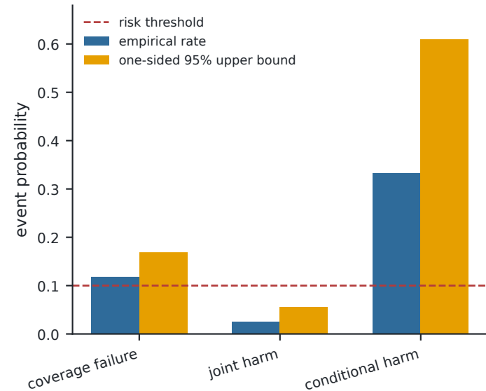
a Hypothetical iid-binomial sensitivity
