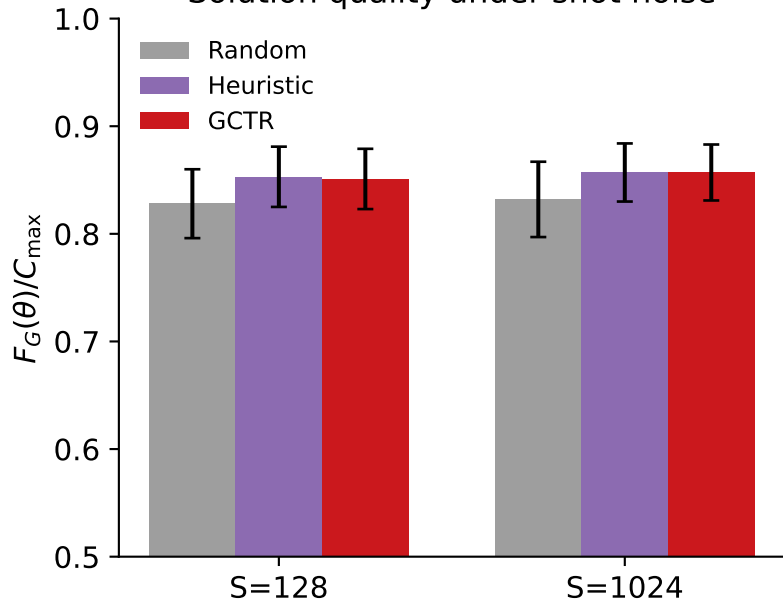
Solution quality under shot noise
