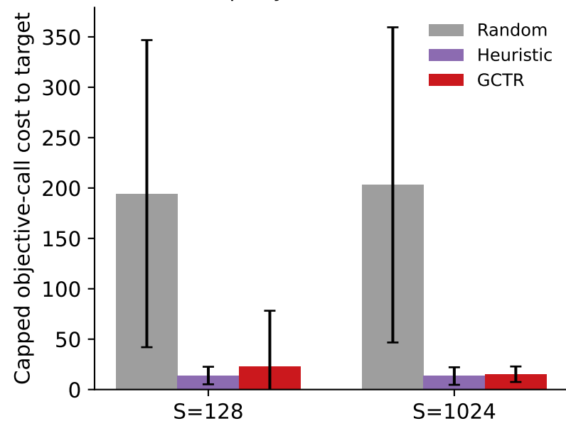
Recorded query count under shot noise
