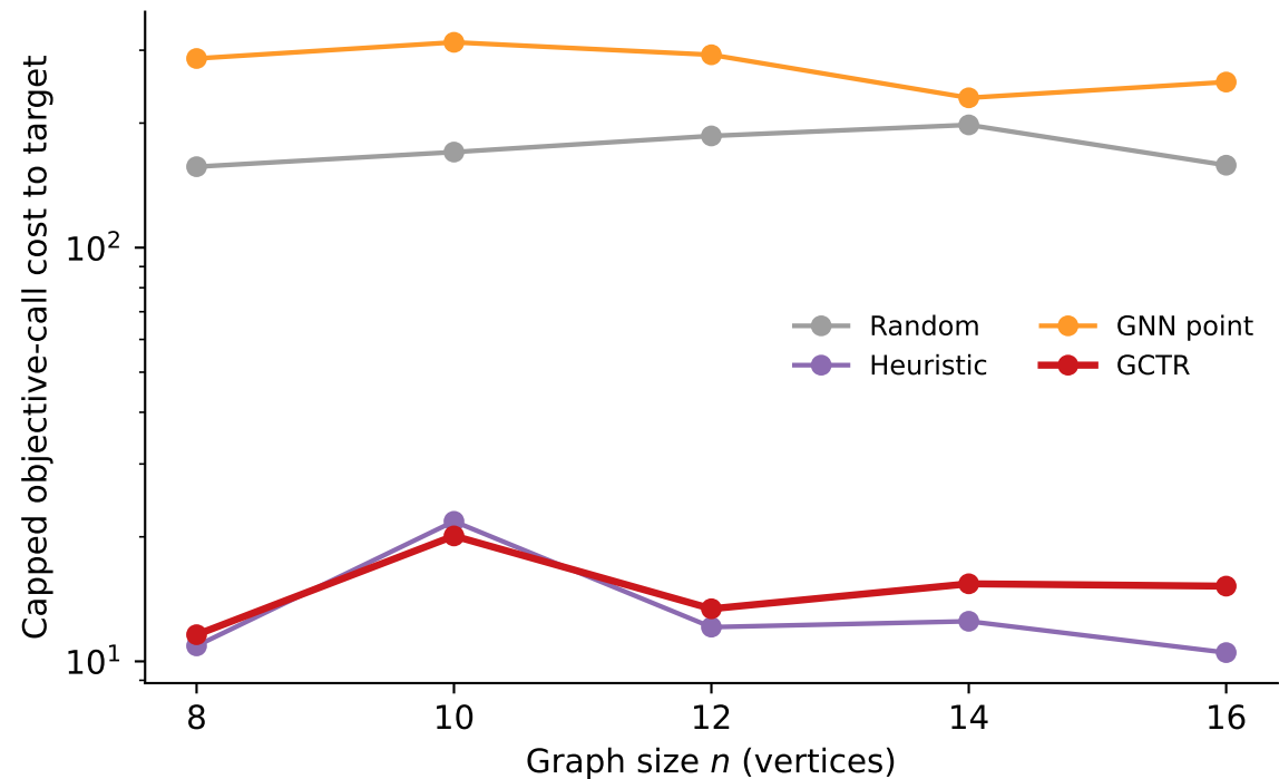
Cross-size transfer (trained at n = 14 )
