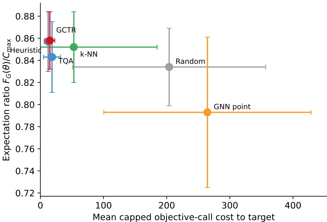
Quality--cost plane at n = 14 (capped cost-to-target protocol)
