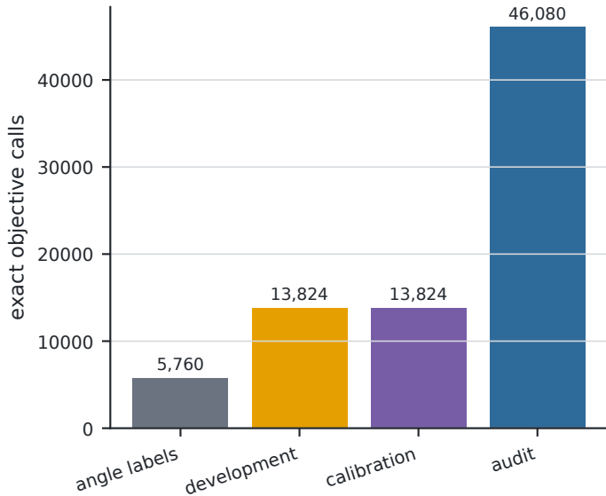
a Offline and audit construction ledger
