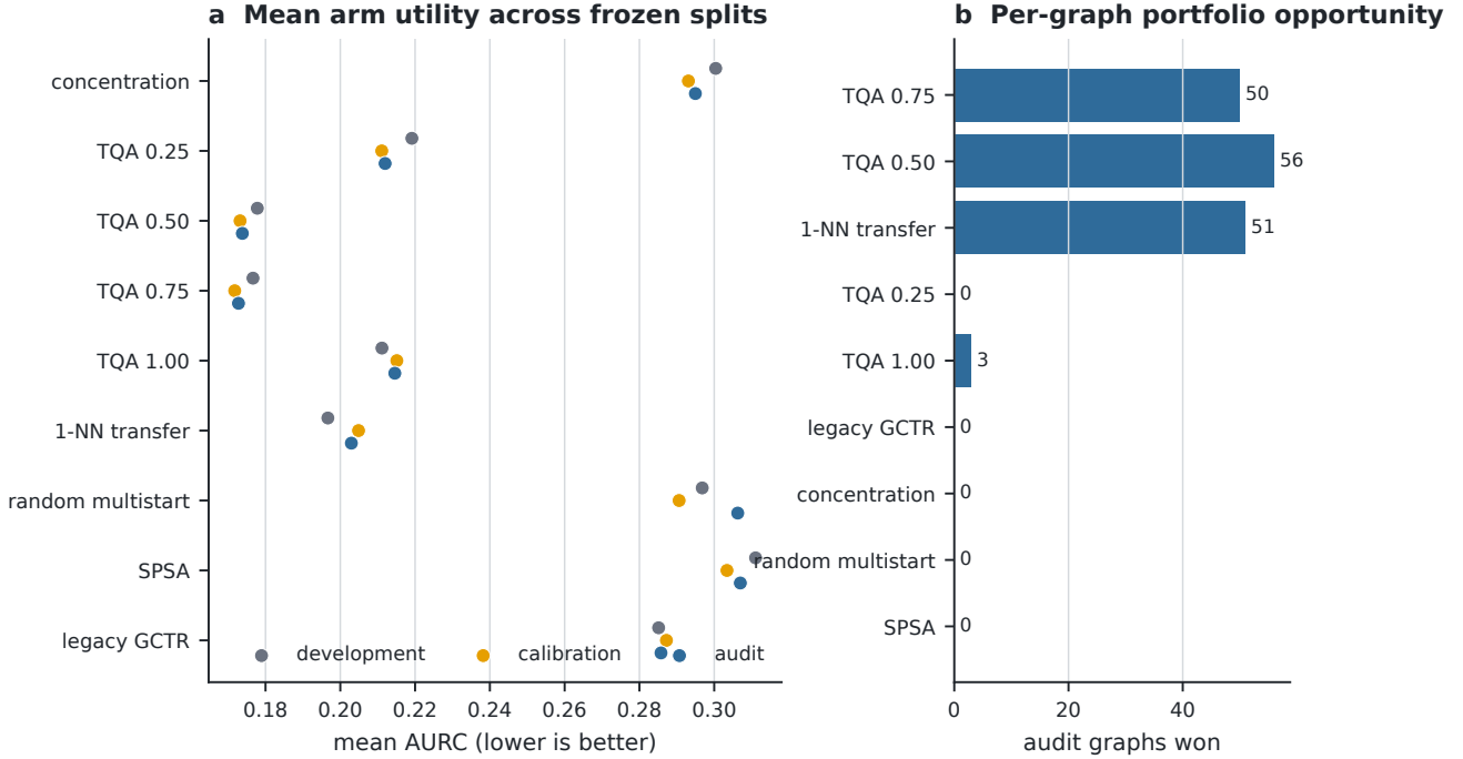
Figure 4: Arm opportunity and split stability. (a) Mean utility for every arm on the frozen development, calibration, and audit splits; lower is better. (b) Number of audit graphs on which each arm is best. Heterogeneous graph-level winners motivate a portfolio but do not by themselves validate a learned router.
