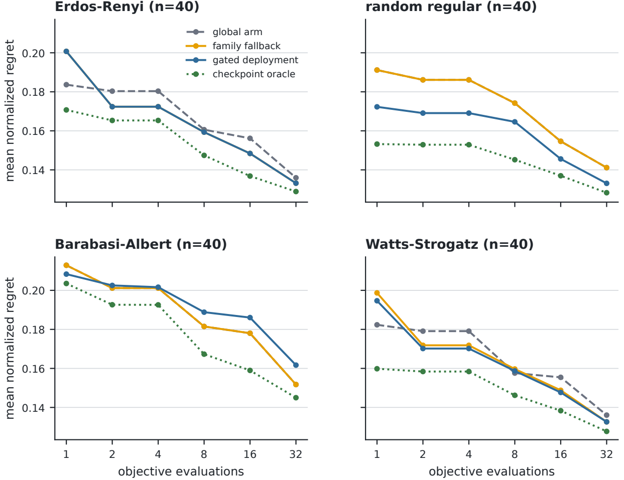
Figure 7: Anytime behavior by fixed graph family. Mean normalized regret is shown at every recorded checkpoint for the global arm, family fallback, gated deployment, and per-checkpoint oracle. Family heterogeneity persists across the 32-call budget.
