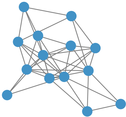
(a) Input graph (ER, n = 14 )
