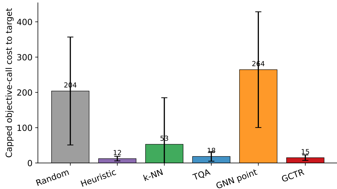
Capped query cost to the 98% target at n = 14 , p = 2 (48 test instances)
