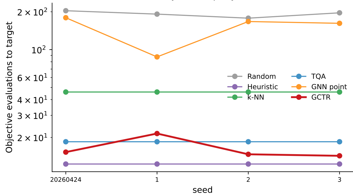
Seed stability of the query benchmark
