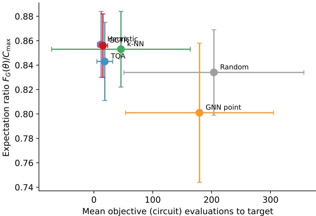
Quality--cost plane at n = 14 (cost-to-target protocol)
