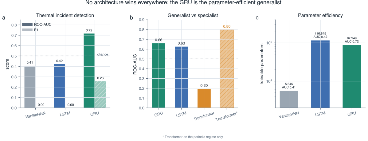
Figure 3. No single architecture wins everywhere. (a) Thermal incident detection: only the GRU exceeds chance-level ranking (ROC-AUC) and produces a non-zero F1. (b) Three-dataset average ROC-AUC; the hatched bar (Transformer*) is the Transformer on the periodic regime only, where it is the overall best. (c) Parameter counts (log scale): the GRU attains the best accuracy with fewer parameters than the LSTM.
