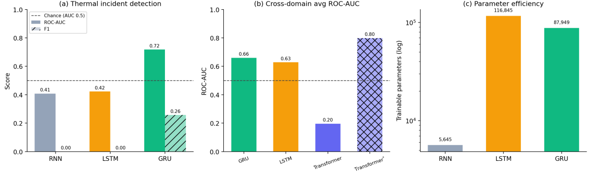
Figure 3. No single architecture wins everywhere. (a) Thermal incident detection: only the GRU exceeds chance-level ranking (ROC-AUC) and produces a non-zero F1. (b) Three-dataset average ROC-AUC; the hatched bar (Transformer*) is the Transformer on the periodic regime only, where it is the overall best. (c) Parameter counts (log scale): the GRU attains the best accuracy with fewer parameters than the LSTM.
