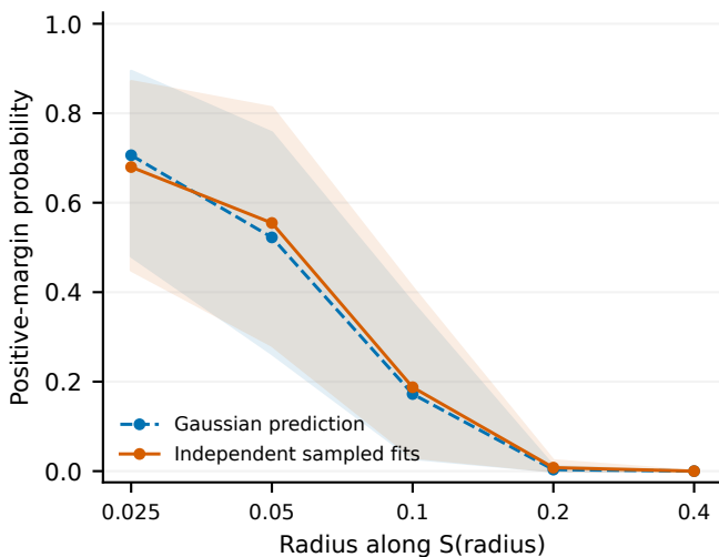
(c) Fresh graphs, p = 2
