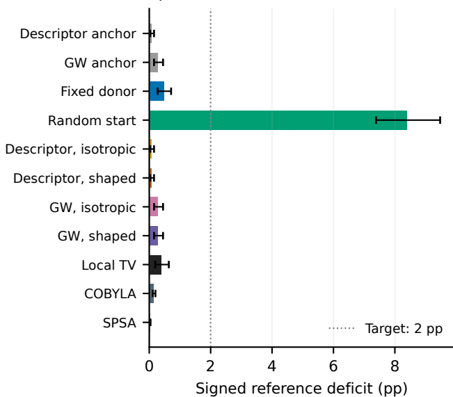
p = 1: competitive methods
