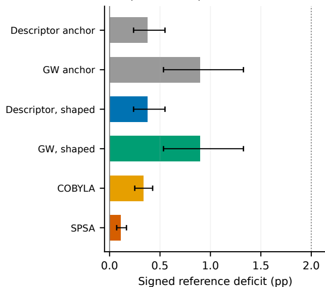
p = 2: competitive methods
