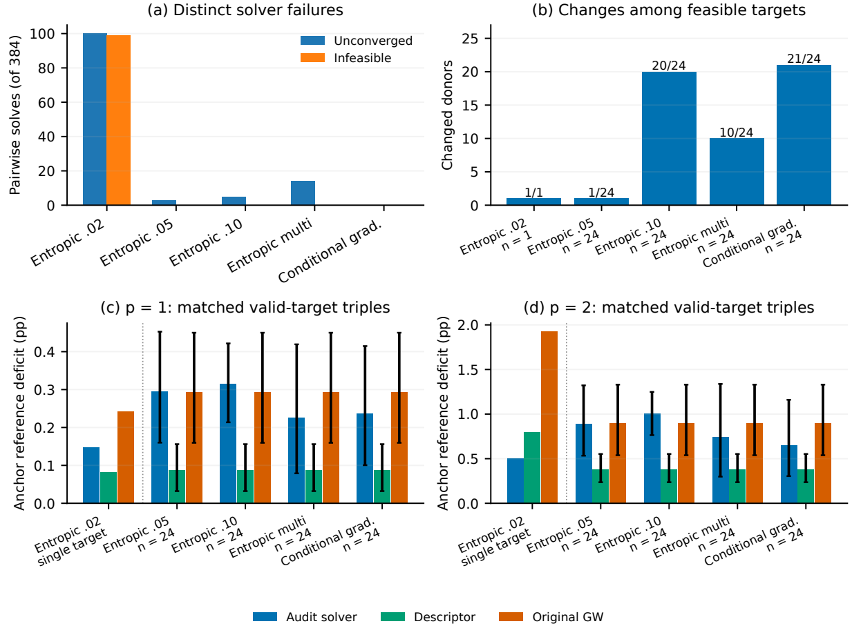
Figure 11: Transport-selector audit. Separate bar panels report solver feasibility and changed donors with explicit target denominators. Quality comparisons use each solver’s common feasible target set and include descriptor and original-solver references. Different solver cohorts do not support a pooled ranking. A one-target cohort is labelled n = 1 and has no across-graph uncertainty interval. The single aggregate audit time is reported in text because per-solver timings are unavailable. The descriptor comparator supplies the inexpensive default used by the revised refinement experiment.
