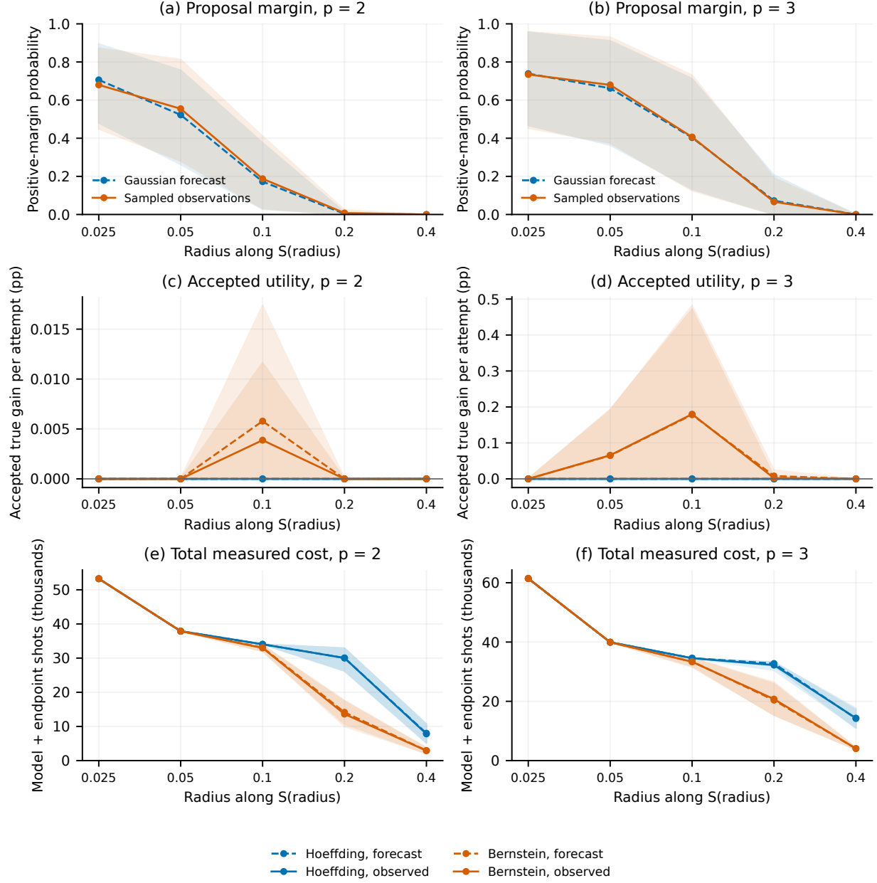
Figure 6: Proposal quality and decision cost on the same allocation schedule. Line panels at depths two and three show positive-margin probability, accepted true gain including zero outcomes, and total model-plus-endpoint shots versus radius. The per-point model counts are 4096, 1024, 256, 64, and 16 at radii 0.025, 0.05, 0.1, 0.2, and 0.4. Every fresh-graph shaped condition contributes 32 sampled-model proposals with eight independent endpoint replays each, and 256 Gaussian proposals with one replay each. Both confidence rules share endpoint streams and use the online L = 4 penalty under a 65536-shot cap. Forecast and observed lines use equal graph weights; pointwise bands resample whole graphs. All signs of the true decrease and margin remain in the denominator. Exact target moments and trial objectives inform the Gaussian population, so its forecast is an offline diagnostic, not a free online decision rule.
