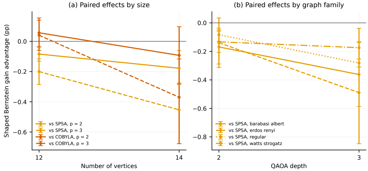
Figure 12: Paired performance across the tested regimes. Lines show the revised policy's gain difference from SPSA and COBYLA across graph sizes (left), and from SPSA across depths within each graph family (right). Zero marks equal gain, and negative effects remain visible. Repetitions are averaged within graphs before uncertainty estimation. Comparisons are conditional on the two existing banks; changing targets across panels prevents an isolated estimate of a bank effect.
