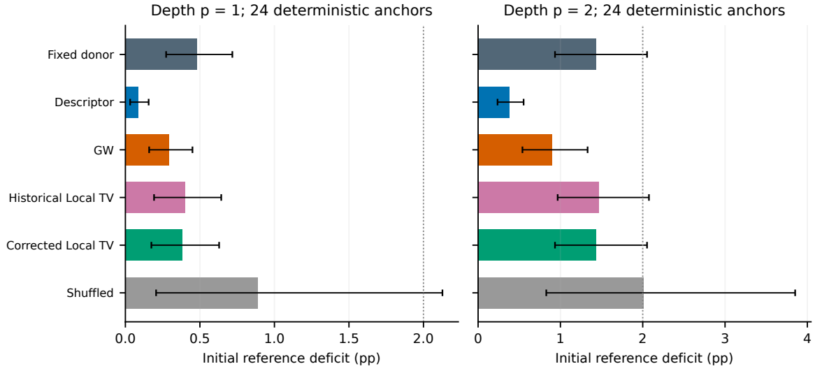
Figure 8: Initial transfer deficits, in percentage points, before target-graph refinement. Bars summarize deterministic initial deficits on 24 graphs; intervals use 10000 graph-bootstrap resamples (95% percentile). Horizontal scales differ between depths. Best-found target references are used only for evaluation. Theorem 1 applies to rooted-neighborhood total variation; the other selectors are heuristic. All depth-two local scores mathematically equal one: the historical Local-TV row retains the floating-point selection artifact, while the corrected deterministic-tie row selects the fixed donor. This separation is not evidence of graph structure.
