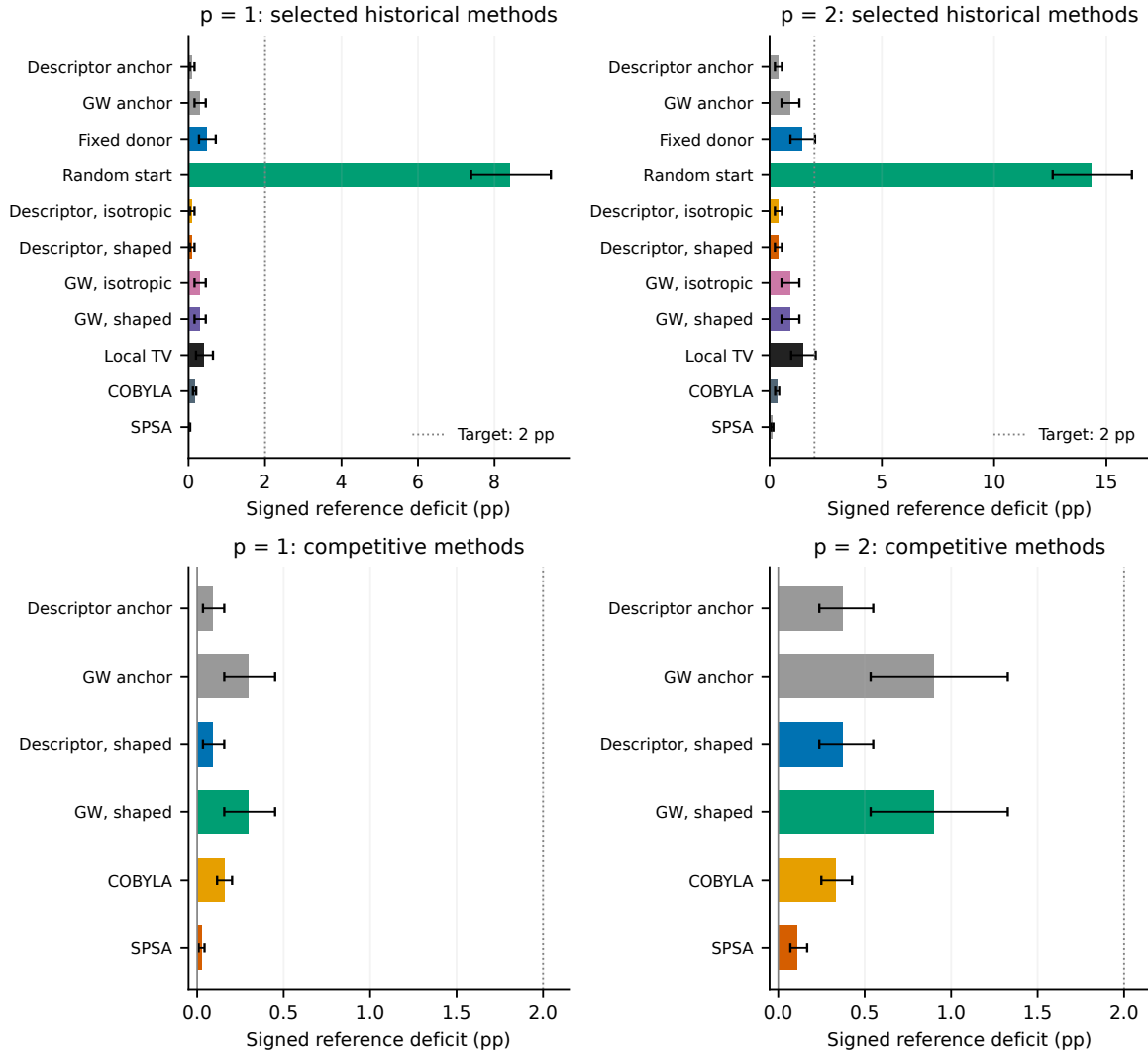
Figure 7: Final quality at a 131072-shot optimization cap, at depths one and two. Deficit is 100 times the signed gap between the returned normalized objective and the best-found reference; smaller is better. The dotted line marks the target gap of 0.02, or two percentage points on the plotted scale. Separate panels show selected historical methods and the competitive methods from a zero origin; initialization-only controls expose the transferred quality. Bars average the 24 graph means after averaging three shot seeds within each graph. Intervals use 10000 graph-bootstrap resamples (95% percentile). Exact objectives are diagnostic; independent final validation is outside the cap.
