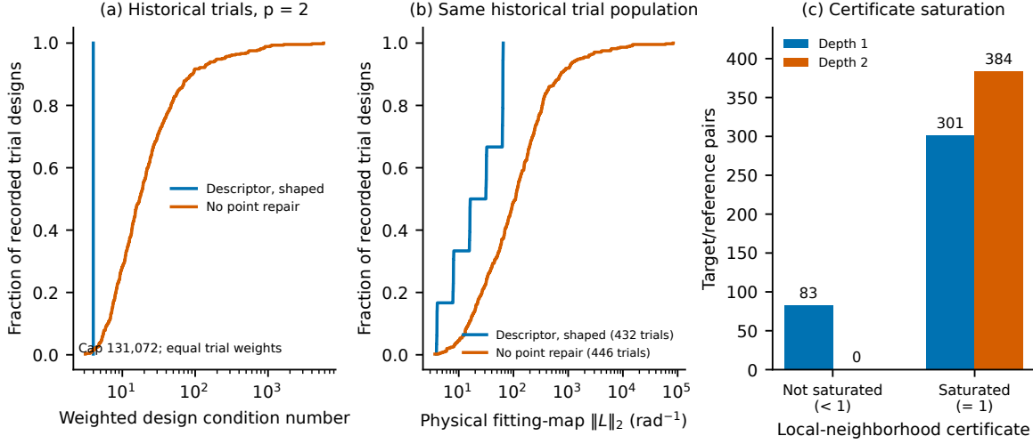
Figure 10: Interpolation geometry, physical sensitivity, and certificate saturation. Step-line empirical cumulative distributions compare recorded weighted-design condition numbers and reconstructed physical gradient fitting-map norms \|L\|_2 for the same 432 repaired and 446 unrepaired models in the depth-two canonical experiment at the 131072-shot cap. Unique unwrapped displacements, unit-ball membership, and agreement with recorded design condition numbers validate each reconstruction. These are executed trial mixtures, whose radii and centers can differ; they do not alone isolate a causal quality effect of point repair. Grouped bars count not-saturated and saturated rooted neighborhood bounds: 83 versus 301 pairs at depth one and 0 versus 384 at depth two. Saturation means total variation one and a vacuous objective bound; a value below one need not be practically useful. The ECDF weights each recorded model equally, so it describes the executed trial mixture rather than giving equal weight to graphs. Good numerical conditioning alone does not establish refinement.
