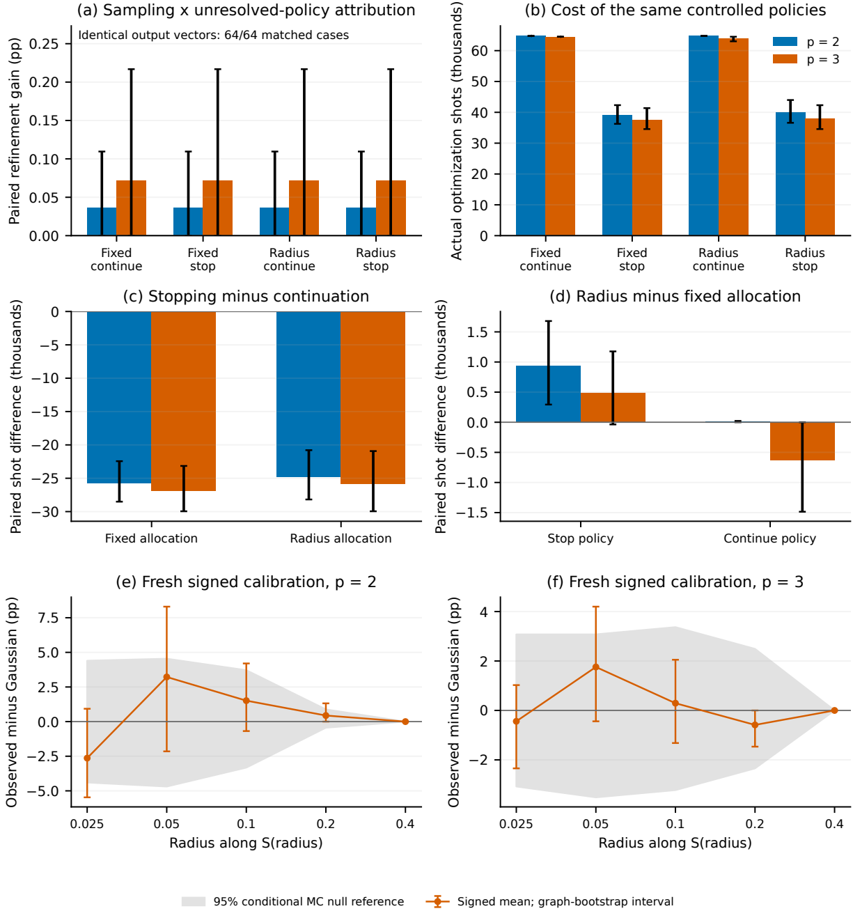
Figure 5: Attribution of expenditure and calibration residuals. Grouped bars report own-anchor gain and optimization shots for the four sampling-by-stopping policies; all four return the same vector in every one of the 64 matched cases. Paired contrasts show stop minus continue and radius-dependent minus fixed allocation, with negative cost differences indicating savings. Continuation refits at the same radius after unresolved evidence. Bottom panels show fresh-graph observed minus Gaussian-predicted positive-margin frequency. Graph-bootstrap intervals and a separate conditional Monte Carlo reference distinguish graph variation from the noise of comparing 32 observed and 256 predicted proposals per condition. The reference assumes equal underlying probabilities within each condition; it is not a bound on Gaussian approximation error. All intervals are pointwise.
