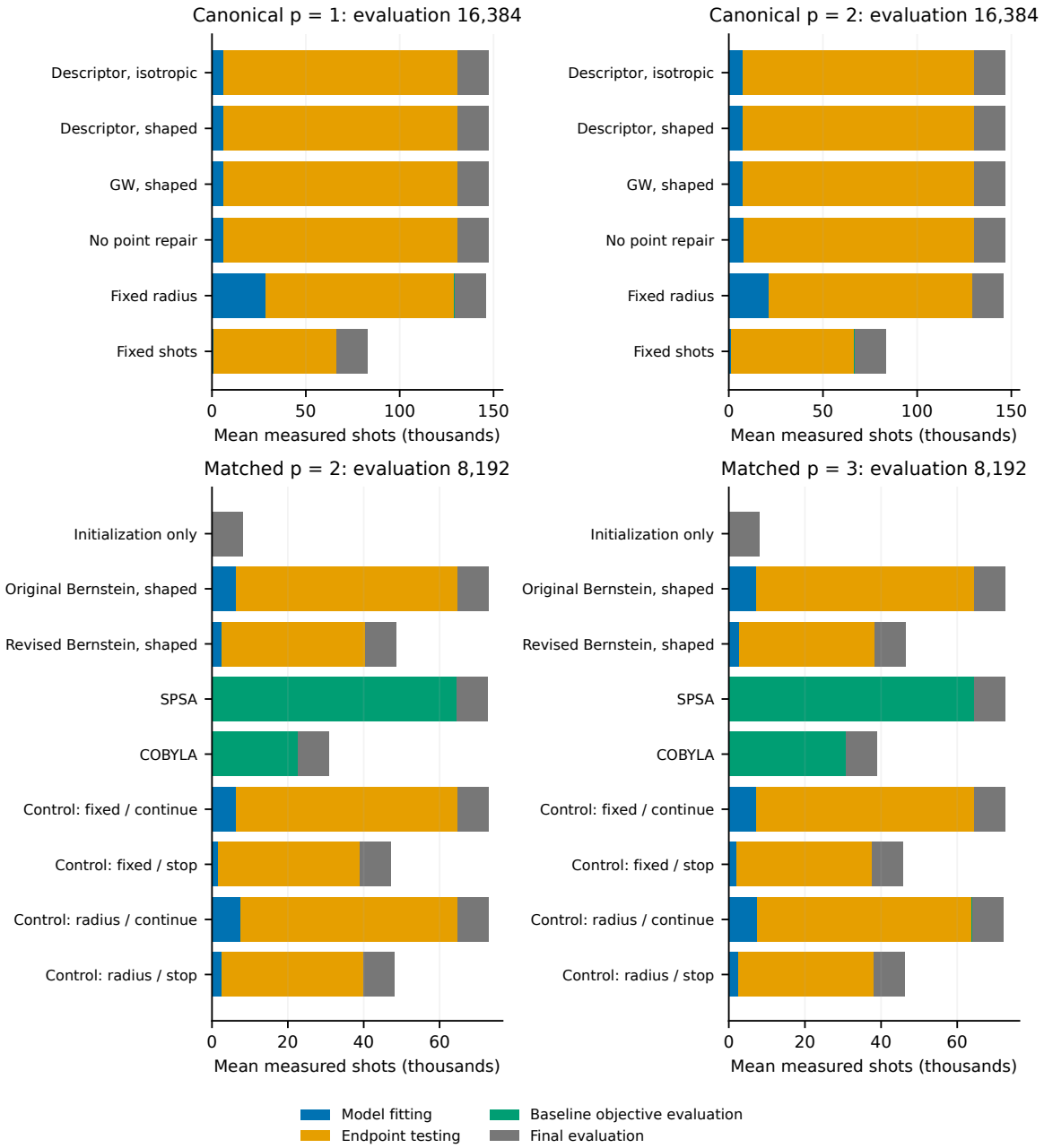
Figure 9: Measurement expenditure across the canonical and matched studies. Stacked bars separate model, acceptance, baseline objective-evaluation, and independent final-evaluation shots. Baseline objective evaluations are the optimization measurements made by SPSA and COBYLA outside the model/test decomposition. Canonical panels use a 131072-shot optimization cap at depths one and two; matched follow-up, shape-by-rule, and sampling-by-stopping panels use a 65536-shot cap at depths two and three. All four attribution policies are retained. Rejected and unresolved trials remain charged. Independent evaluation costs 16384 shots per canonical run and 8192 per matched run. These bars report expenditure rather than optimization trajectories.
