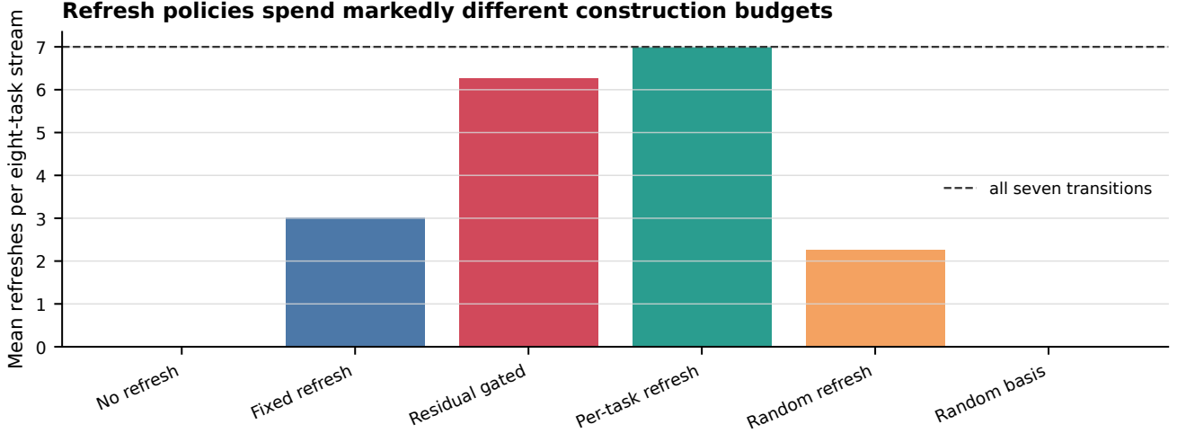
Extended Data Figure 3: Refresh burden. The residual gate rebuilds on most of the seven transitions, whereas fixed and random controls spend smaller construction budgets.
