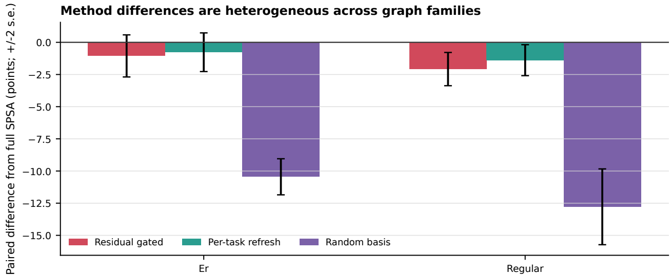
Extended Data Figure 6: Family heterogeneity. Paired method differences vary across the configured graph generators; bars show descriptive \pm 2 standard errors.
