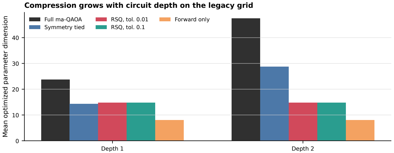
Extended Data Figure 4: Depth-dependent compression. The number of retained directions grows more slowly than the ambient multi-angle dimension on this small legacy grid.
