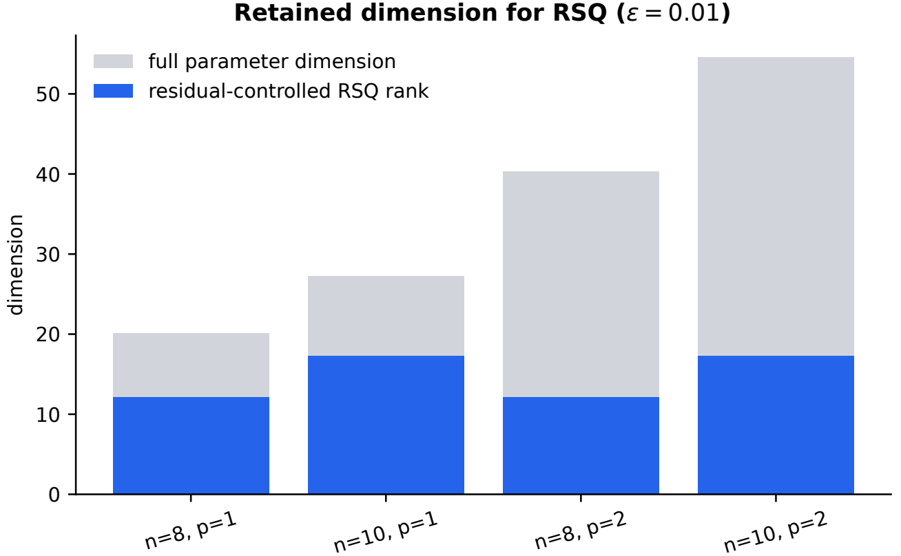
Extended Data Figure 2: Selected rank across the legacy grid. Rank adapts to the local sensitivity spectrum but does not by itself predict end-to-end efficiency.
