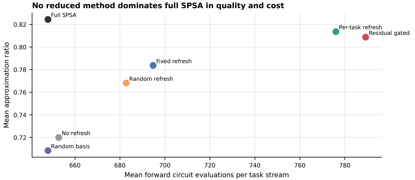
Extended Data Figure 5: Quality-cost frontier. Mean forward cost includes scalar and vector-observable points. No reduced method simultaneously dominates full SPSA in the development audit.
