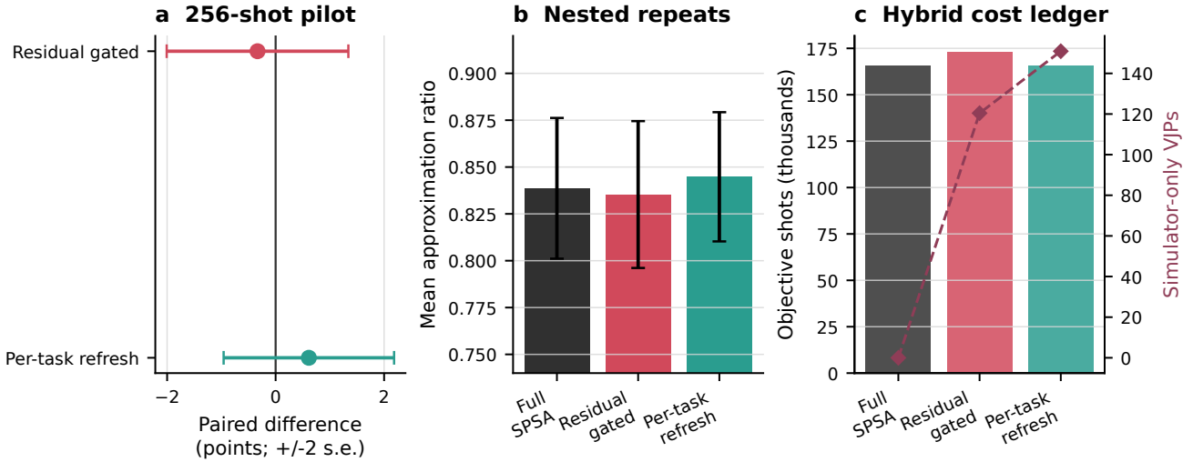
Figure 4: Finite-shot objective pilot. Scalar objectives use 256 shots, while subspace construction uses exact simulator observables and VJPs. Reported approximation ratios are exact post-evaluations of parameters selected with sampled objectives. This is not an end-to-end hardware experiment.
