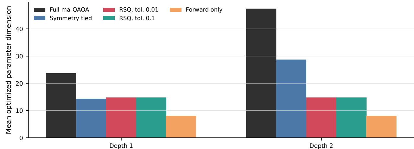
Compression grows with circuit depth on the legacy grid
