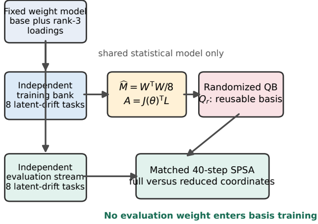
FIG. 1. Leakage-resistant repeated-task protocol. A training bank defines the empirical task second moment; an independent evaluation stream tests transfer. Randomized QB constructs a local basis from J^T L , and full and reduced SPSA receive the same 40-step schedule. The displayed development decision is generated from the committed evidence.
