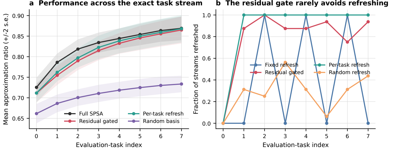
FIG. 2. Evaluation-task trajectories. The left panel reports task-index performance after nesting repeated measurements within a graph-depth cell. The right panel shows that residual gating refreshes on most eligible transitions, limiting amortization in the tested regime.
