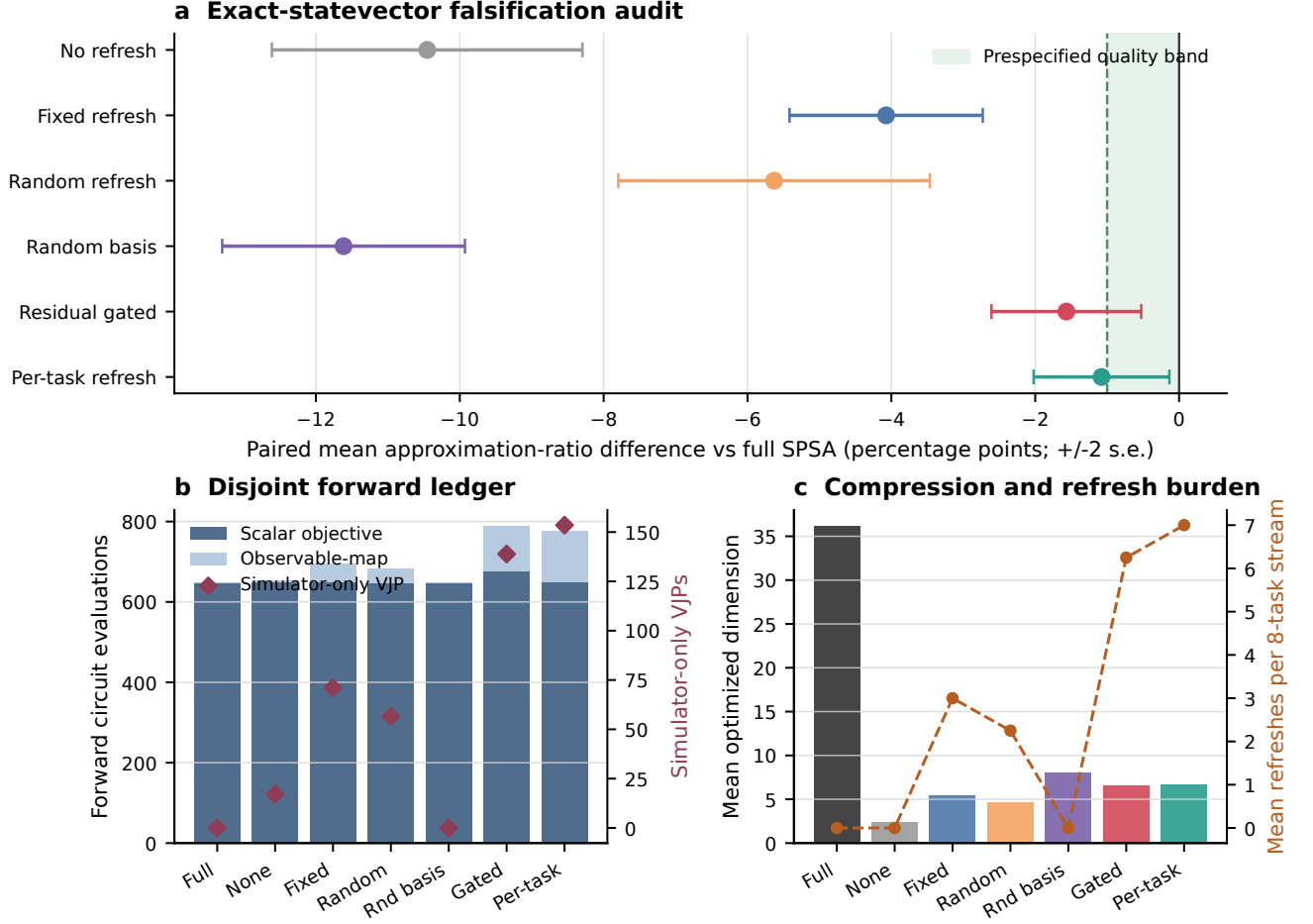
FIG. 3. Exact-statevector falsification audit. Residual-gated reuse misses the declared one-percentage-point quality band and spends additional observable evaluations and simulator VJPs. Error bars are descriptive \pm 2 standard errors over configured graph-depth cells.
