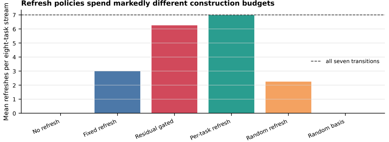
FIG. 9. Refresh burden. The residual gate rebuilds on most of the seven transitions, whereas fixed and random controls spend smaller construction budgets.
