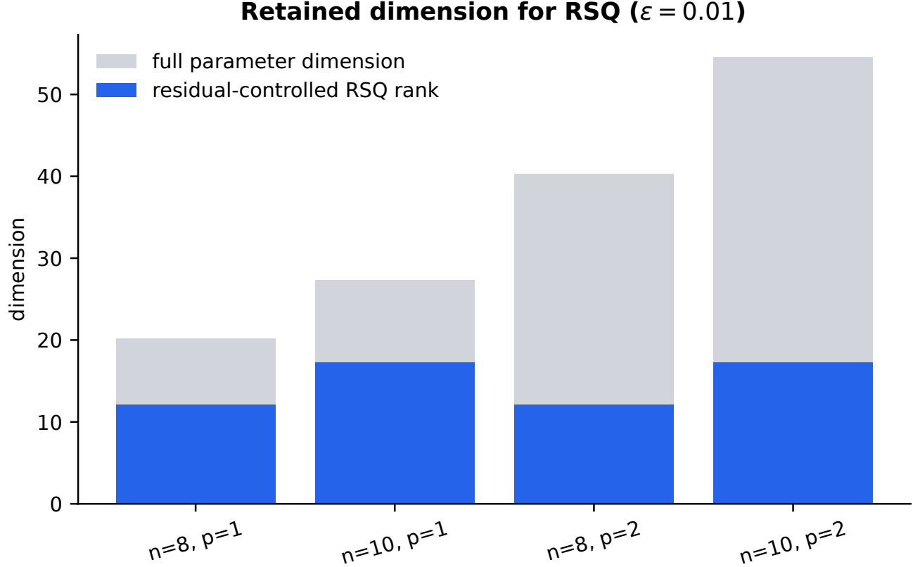
FIG. 8. Selected rank across the legacy grid. Rank adapts to the local sensitivity spectrum but does not by itself predict end-to-end efficiency.
