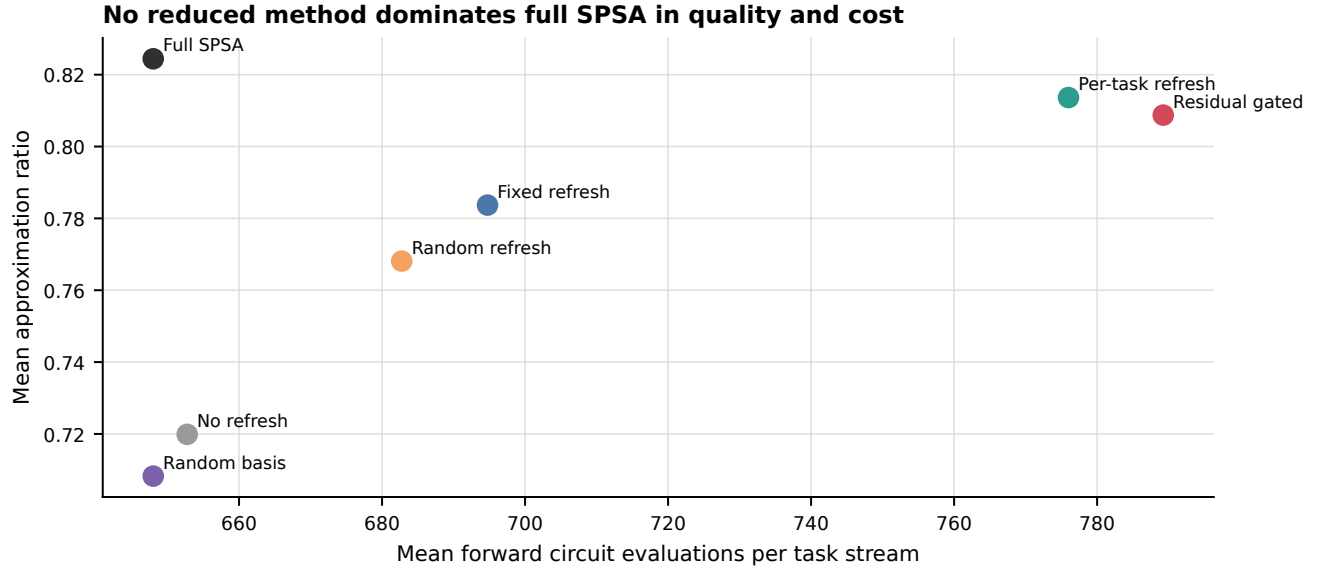
FIG. 11. Quality-cost frontier. Mean forward cost includes scalar and vector-observable points. No reduced method simultaneously dominates full SPSA in the development audit.
