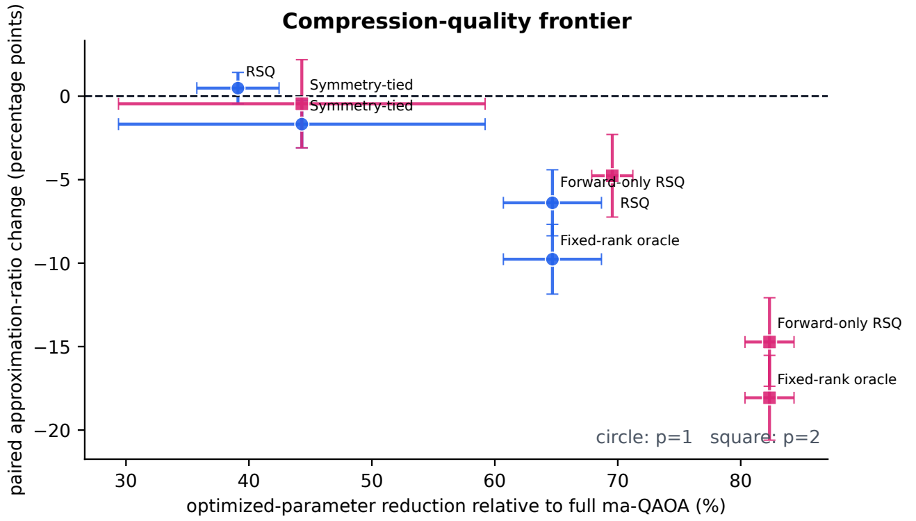
FIG. 4. Legacy compression-quality tradeoff. The figure preserves the original exact-statevector evidence track and exposes the stronger depth dependence that motivated the repeated-task audit.
