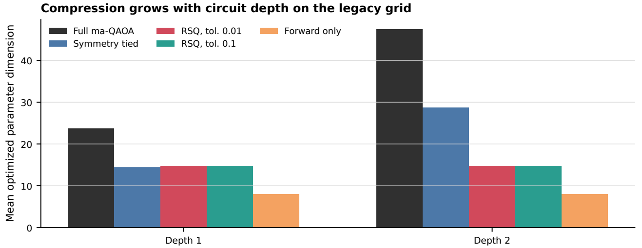
FIG. 10. Depth-dependent compression. The number of retained directions grows more slowly than the ambient multi-angle dimension on this small legacy grid.
