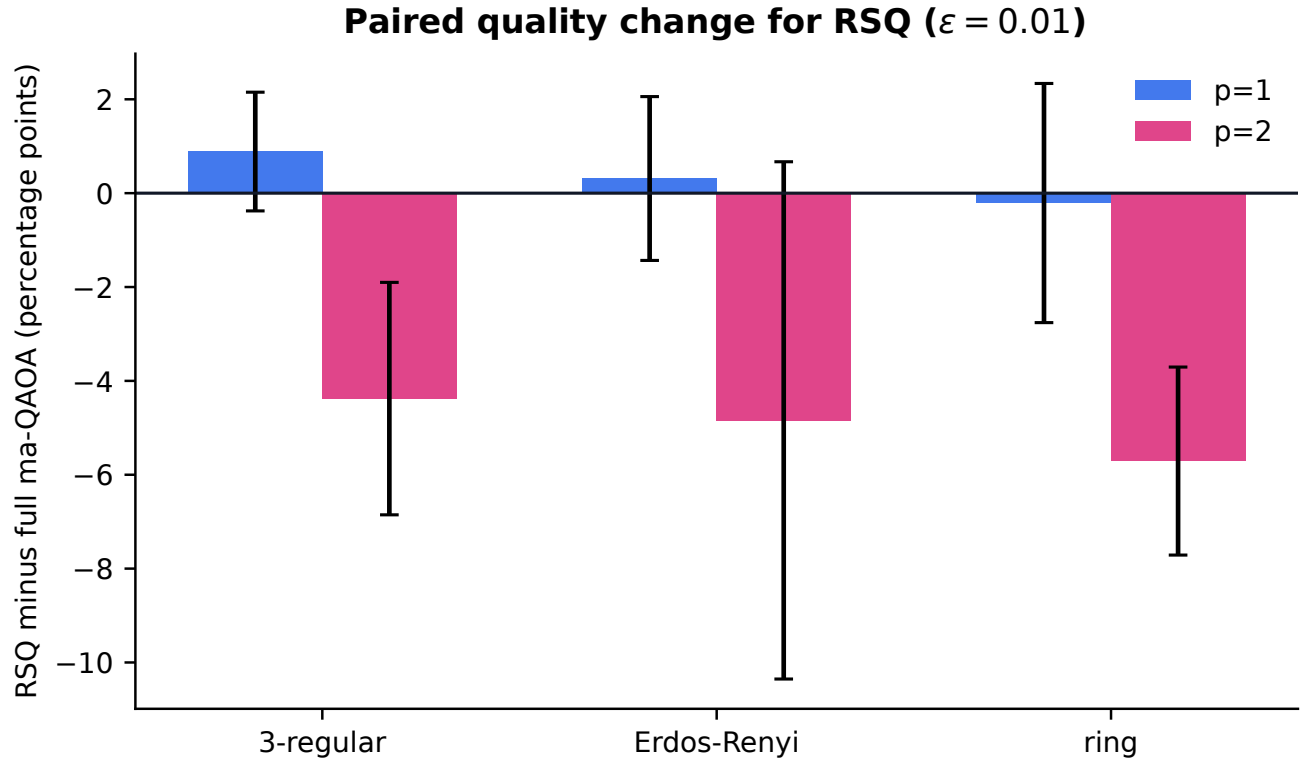
FIG. 6. Legacy family-stratified behavior. Performance depends on graph family and depth, so pooled averages are accompanied by stratified diagnostics.
