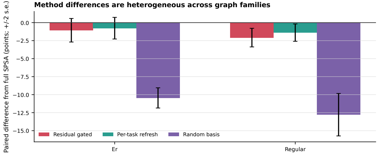
FIG. 12. Family heterogeneity. Paired method differences vary across the configured graph generators; bars show descriptive \pm 2 standard errors.
