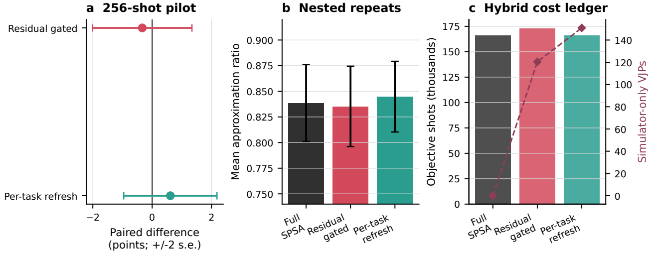
FIG. 5. Finite-shot objective pilot. Scalar objectives use 256 shots, while subspace construction remains exact and simulator-assisted. Consequently, the figure is not an end-to-end hardware experiment.
