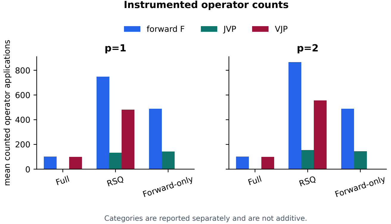
FIG. 7. Operator-access ledger. Forward observable evaluations, finite-difference JVPs, simulator VJP, and dense-Jacobian events are reported as distinct quantities.
