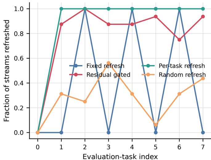
b The residual gate rarely avoids refreshing
