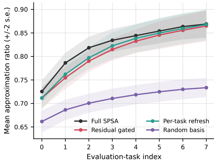
a Performance across the exact task stream
