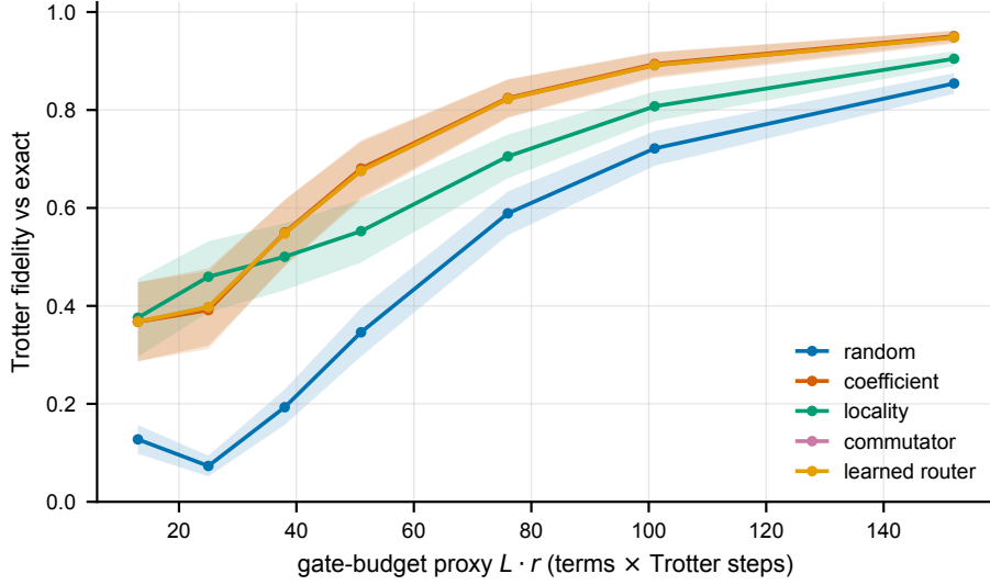
Figure 2: Fidelity versus gate-budget proxy ( L \cdot r ) for the five term orderings as the Trotter step count sweeps \{1, 2, 3, 4, 6, 8, 12\} . Lines are means over the n = 120 instances; shaded bands are 95% confidence intervals ( 1.96 s/\sqrt{n} ) on each mean. Random ordering is dominated at every budget; the non-random orderings are nearly coincident (their bands overlap), consistent with the within-noise reading of Table 1.
