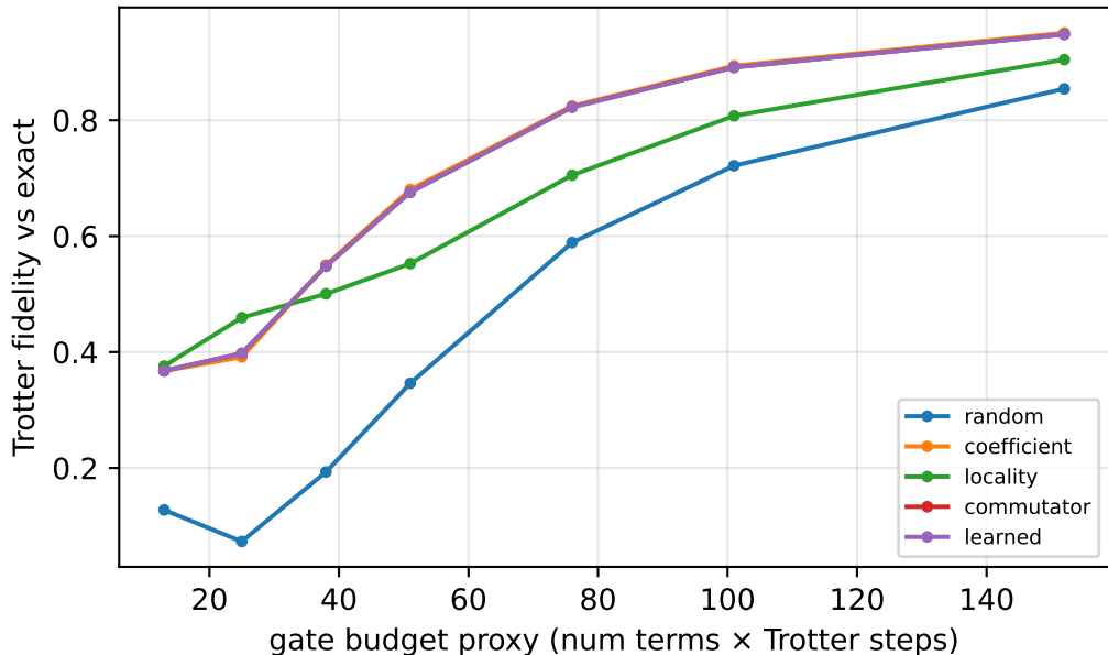
First-order Trotter: term-ordering policies
