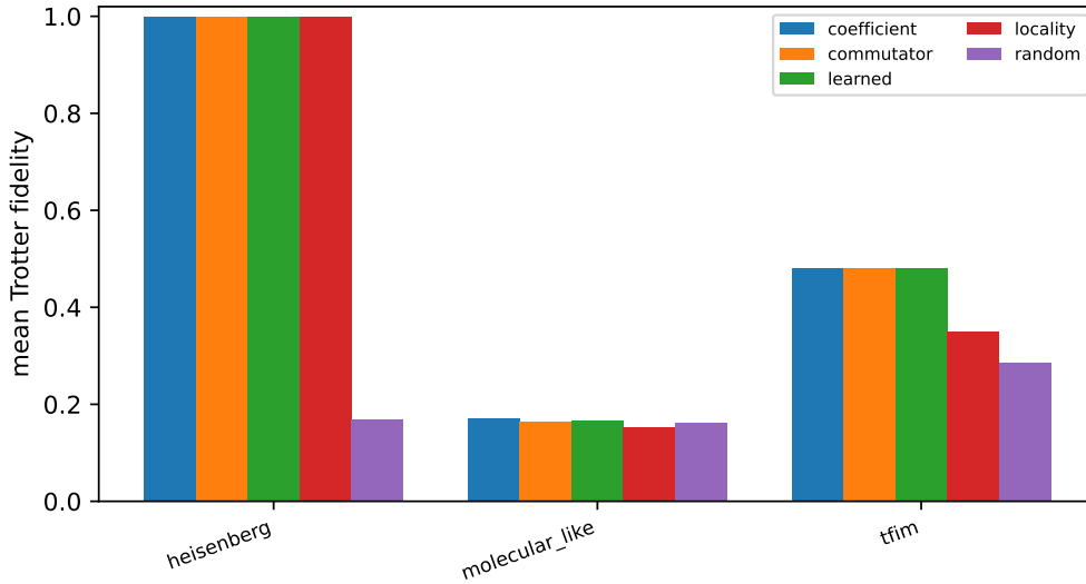
Figure 2: Mean Trotter fidelity by Hamiltonian family for each ordering (reported scale). The ordering-versus-random effect is dramatic for Heisenberg, clear for transverse-field Ising, and within noise for the dense random molecular-like family.
