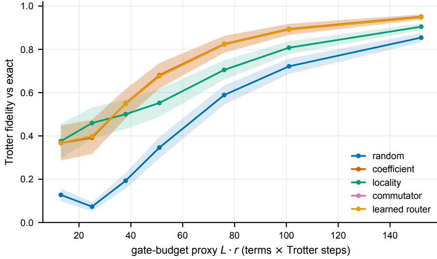
Figure 2: Fidelity-gate-budget frontier across term orderings. Fidelity versus gate-budget proxy ( L \cdot r ) for the five term orderings as the Trotter step count sweeps \{1, 2, 3, 4, 6, 8, 12\} . Lines are means over the n = 120 instances; shaded bands are 95% confidence intervals ( 1.96 s / \sqrt{n} ) on each mean, where s is the sample standard deviation. Random ordering is dominated at every budget; the non-random orderings are nearly coincident (their bands overlap), consistent with the within-noise reading of Table 1.
