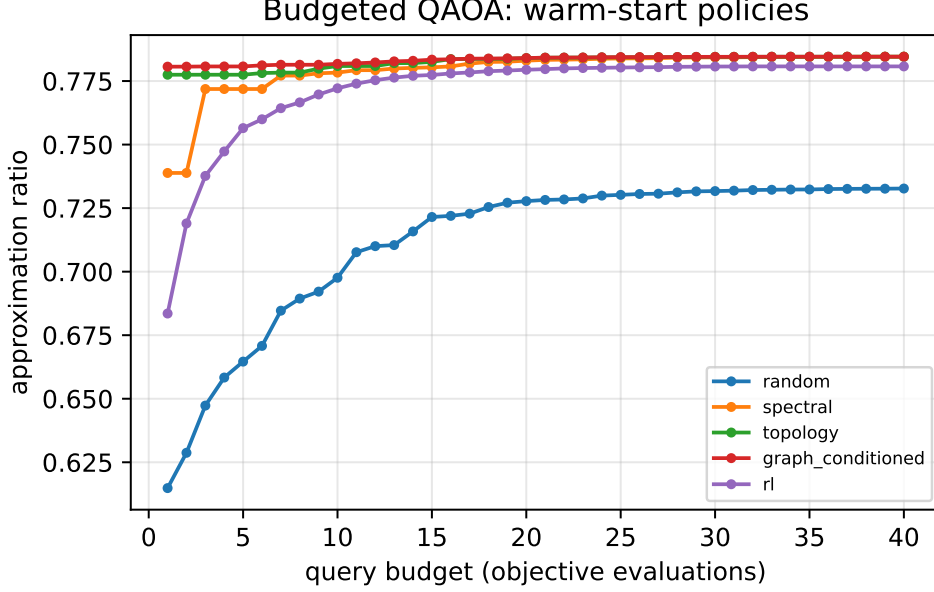
Figure 1. Budgeted QAOA warm-start frontier. Mean running-best approximation ratio (averaged over all 120 held-out test graphs) versus query budget, one curve per warm-start policy. Structure-aware policies (spectral, topology, graph-conditioned) begin far above random and converge onto a common ratio near 0.7846 as the refiner spends its budget; random initialization trails throughout, ending at 0.7327. The learned graph-conditioned policy’s early-budget edge is erased by the local refiner, so its final ratio coincides with the spectral baseline. Data: the frontier block of results/summary.json .
