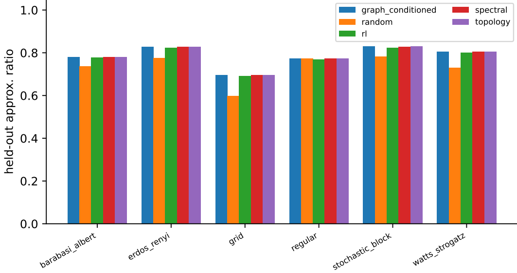
Figure 2. Held-out approximation ratio by graph family. Grouped bars show the mean held-out ratio for each policy within each of the six families ( n = 20 per family); for each family the graph-conditioned policy is fit only on the other five families. The three structure-aware policies are nearly superimposed in every family; cross-family differences (easiest on stochastic-block and Erdős–Rényi, hardest on grids) dominate over policy differences, and all structure-aware policies improve on random everywhere, most where random is weakest (grid, Watts–Strogatz). Data: the by_family block of results/summary.json .
