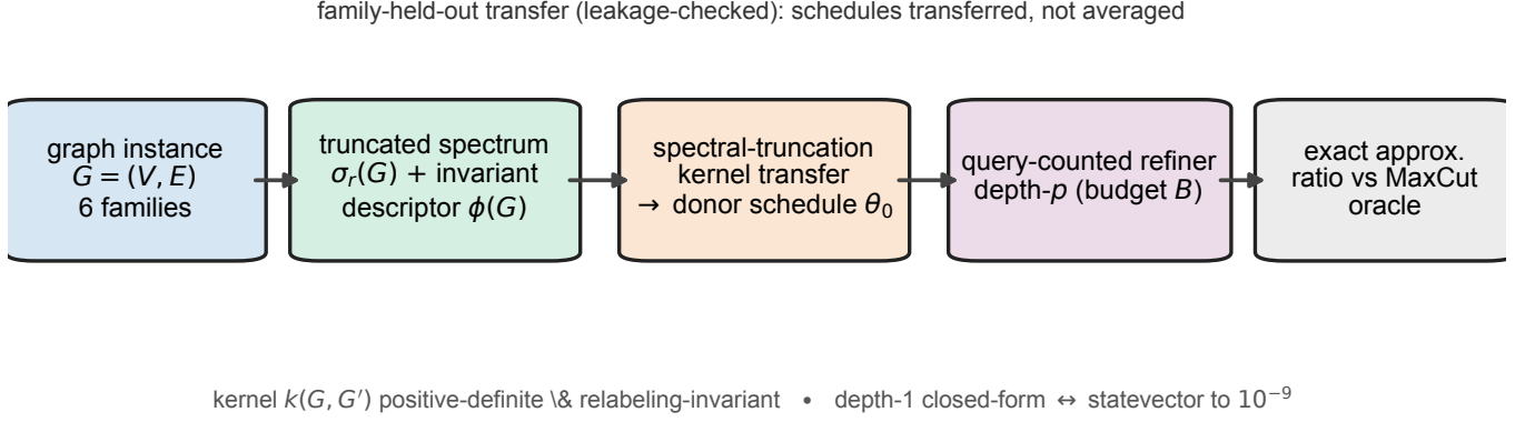
FIG. 1. Spectral-truncation-kernel schedule transfer for QAOA warm starts. A connected graph from one of six families is mapped to a relabeling-invariant representation: a truncated normalized-Laplacian spectrum \sigma_r(G) , a finite low-frequency window of the graph operator, together with an invariant topology descriptor \phi(G) . A positive-definite spectral-truncation kernel k(G, G') selects the single most similar training graph and copies its optimized depth- p angle schedule \theta_0 , transferring one real optimum rather than averaging several. The schedule seeds a refiner that counts every objective evaluation against a fixed budget B ; quality is the exact approximation ratio against a brute-force MaxCut oracle. Two guarantees underpin the benchmark: the kernel is positive definite and invariant, k(\pi G, \cdot) = k(G, \cdot) , and the depth-one objective is computed in two independent ways, an analytic closed form and an exact statevector simulation, agreeing to 10^{-9} . Policies are compared under family-held-out splits with a programmatic leakage check.
