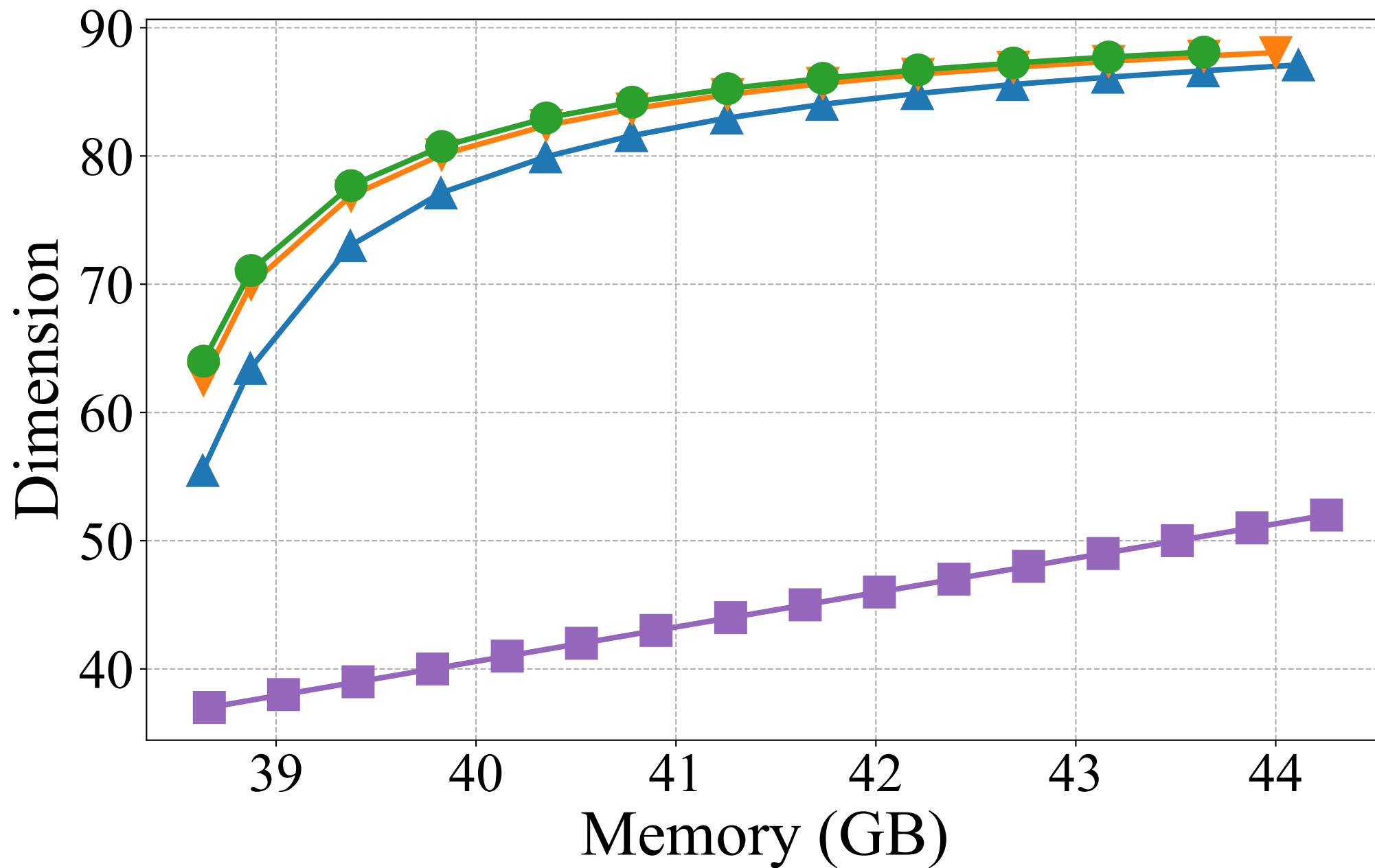
DEEP100M
