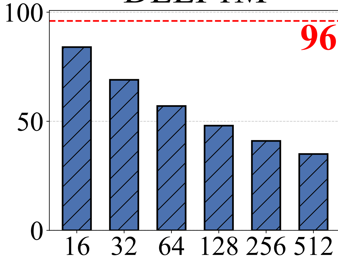
DEEP1M
