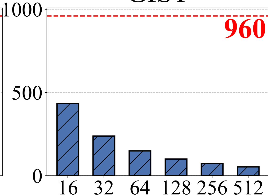
GIST
