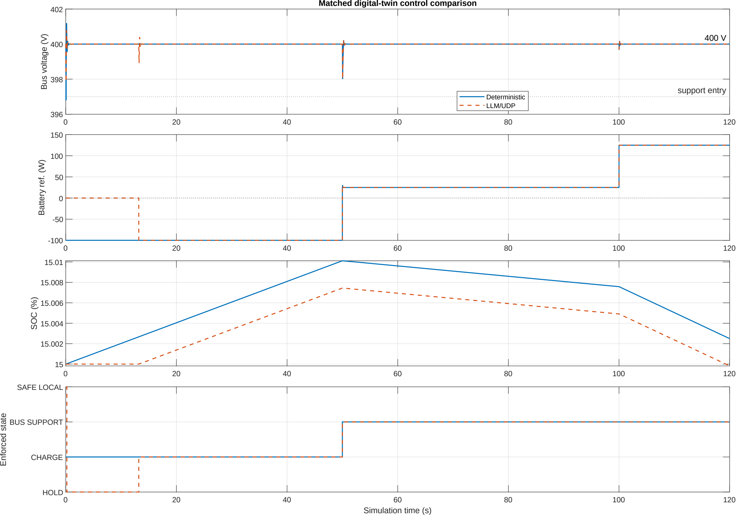
Matched digital-twin control comparison
