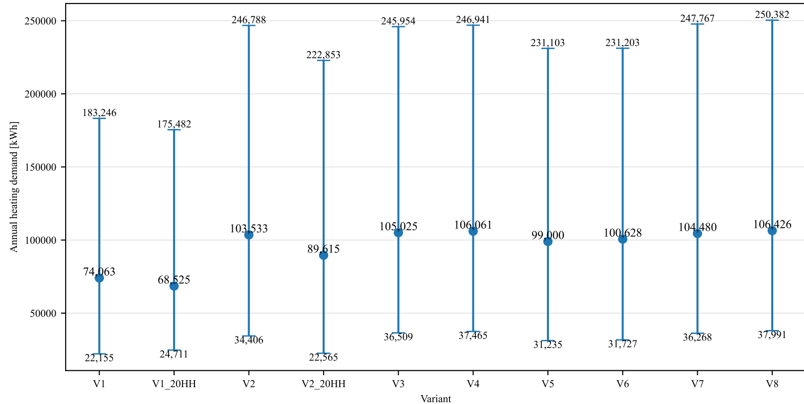
Annual heating demand: P5 / P50 / P95 across all runs
