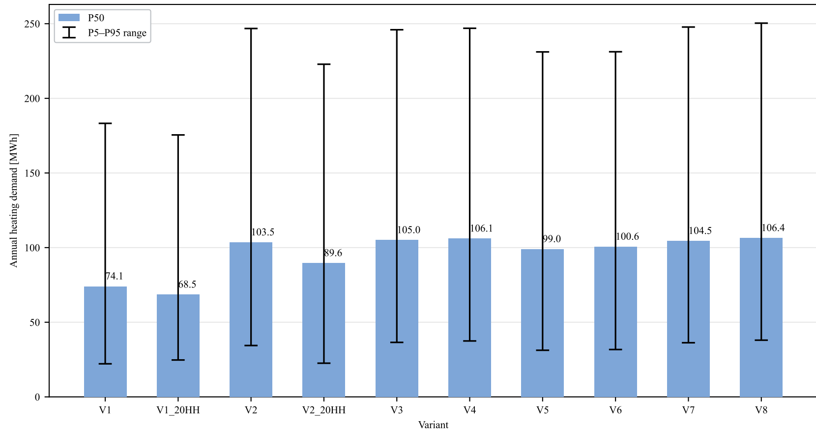
Annual heating demand by variant (P50 with P5/P95 error bars)
