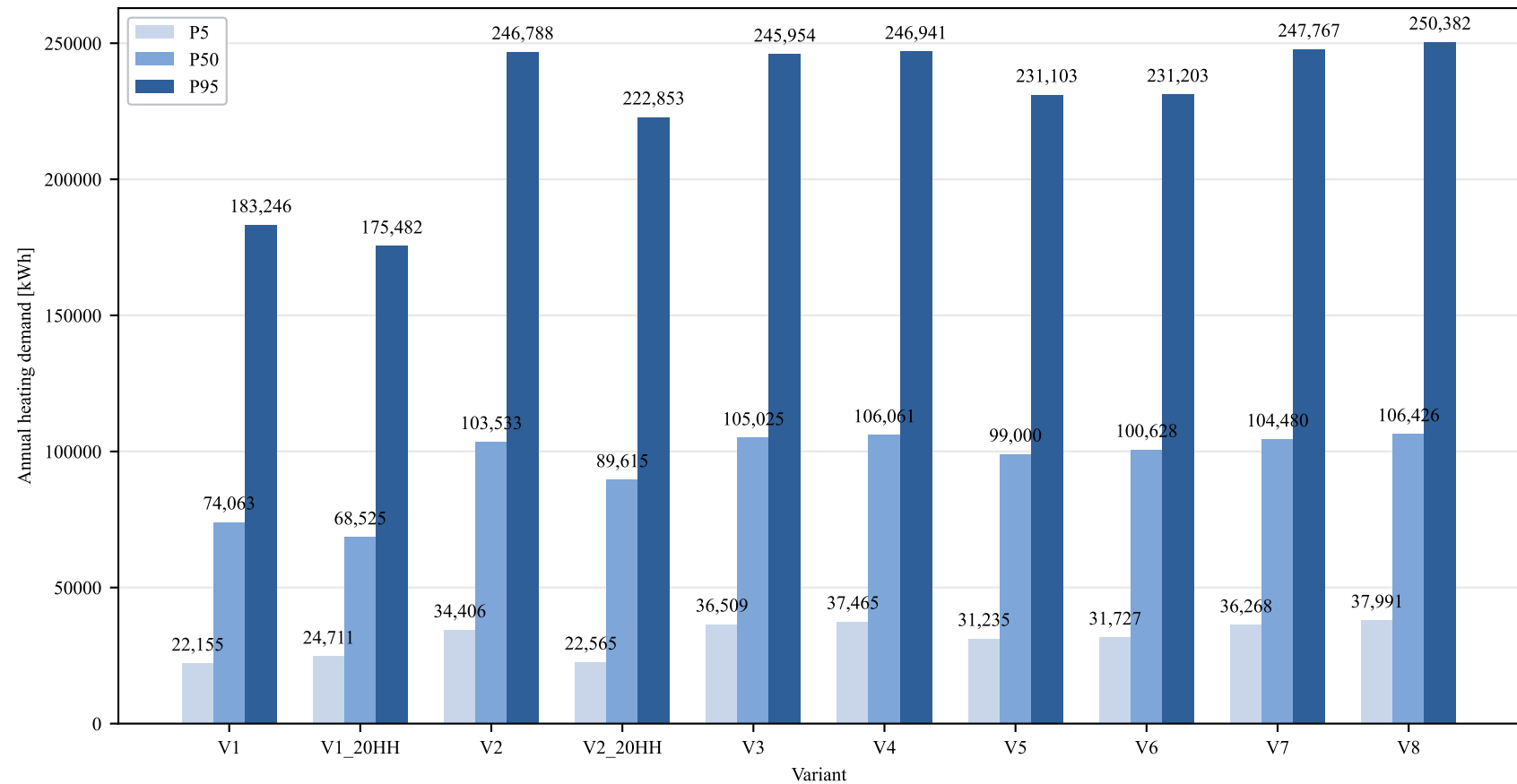
Annual heating demand by variant: P5 / P50 / P95
