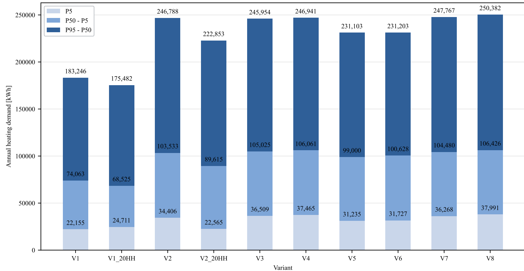
Annual heating demand by variant: stacked quantile band
