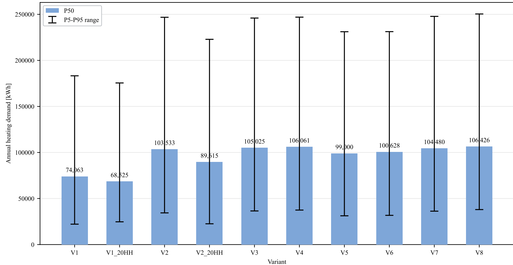
Annual heating demand by variant: P50 with P5/P95 range
