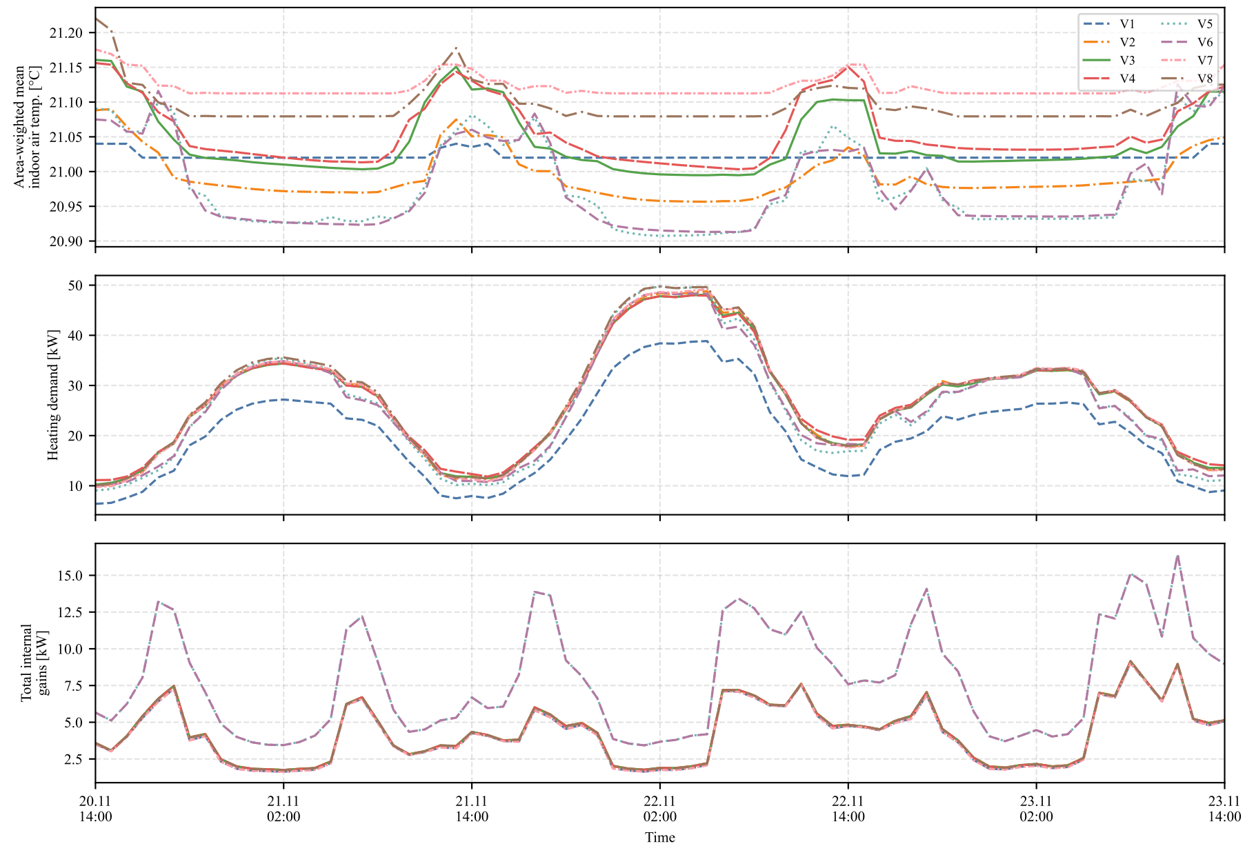
3-day peak heating event window around 2021-11-22 02:00
