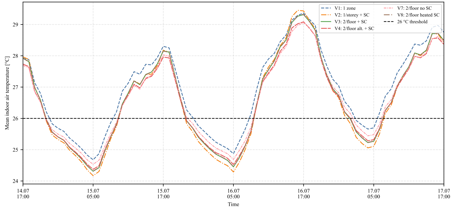
3-day worst overheating window
