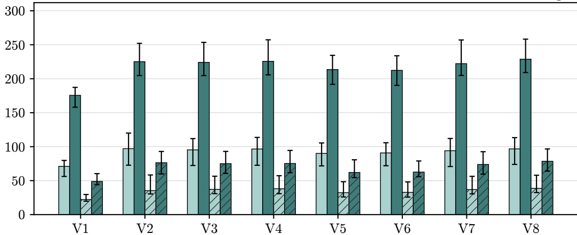
Annual heating demand in MWh
