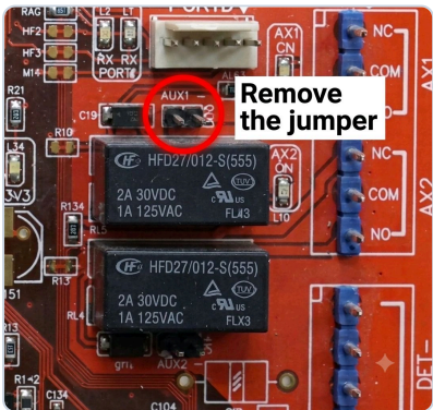
AUX1 relay header — EOL jumper shown, remove it
