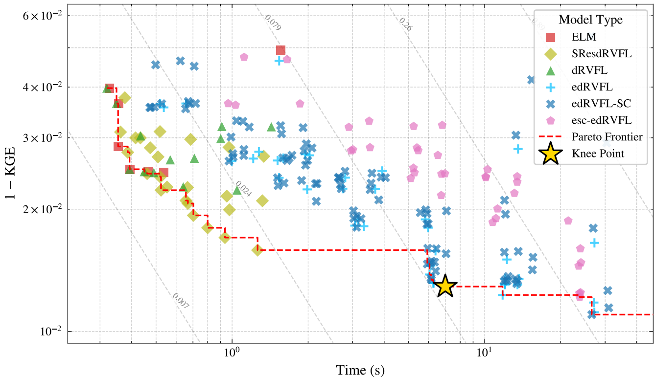
1 - KGE vs. Training Time — Cone
