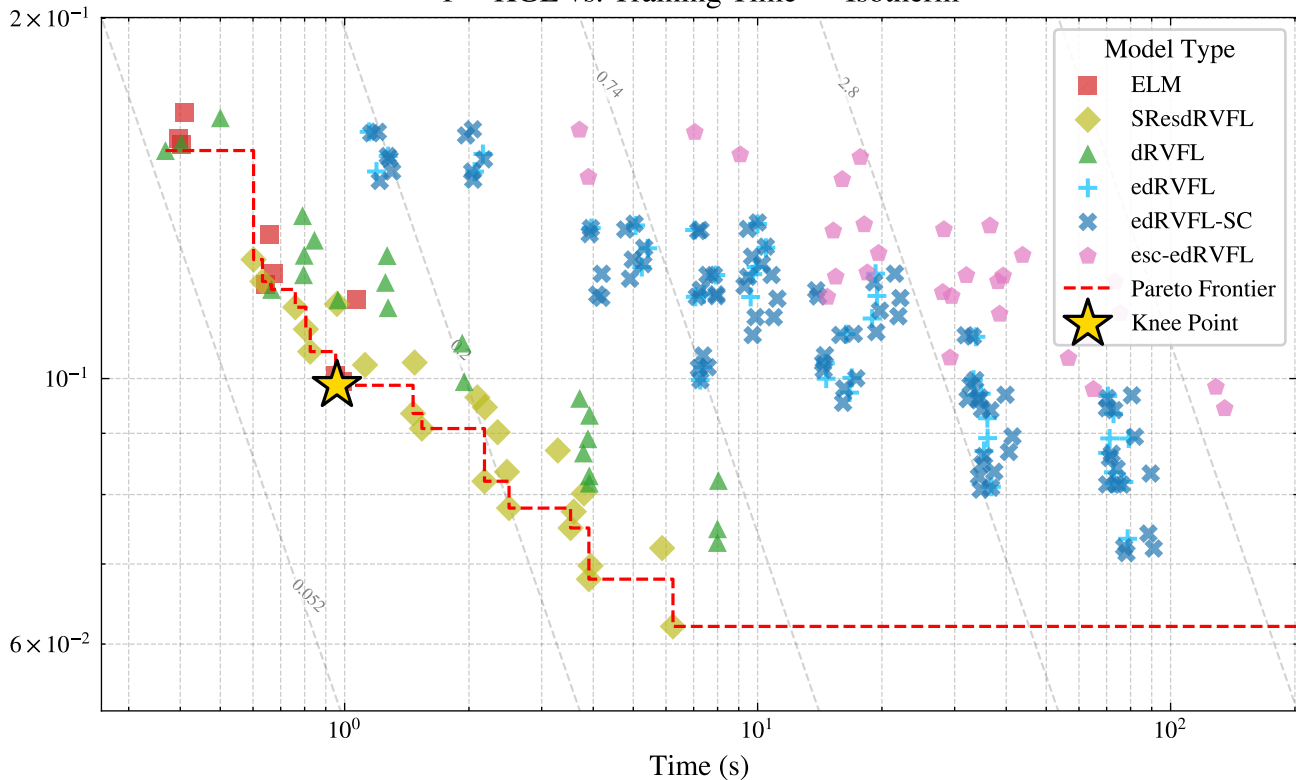
1 - KGE vs. Training Time — Isotherm
