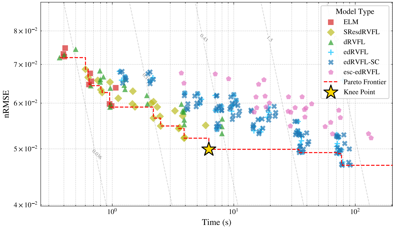
nRMSE vs. Training Time — Isotherm
