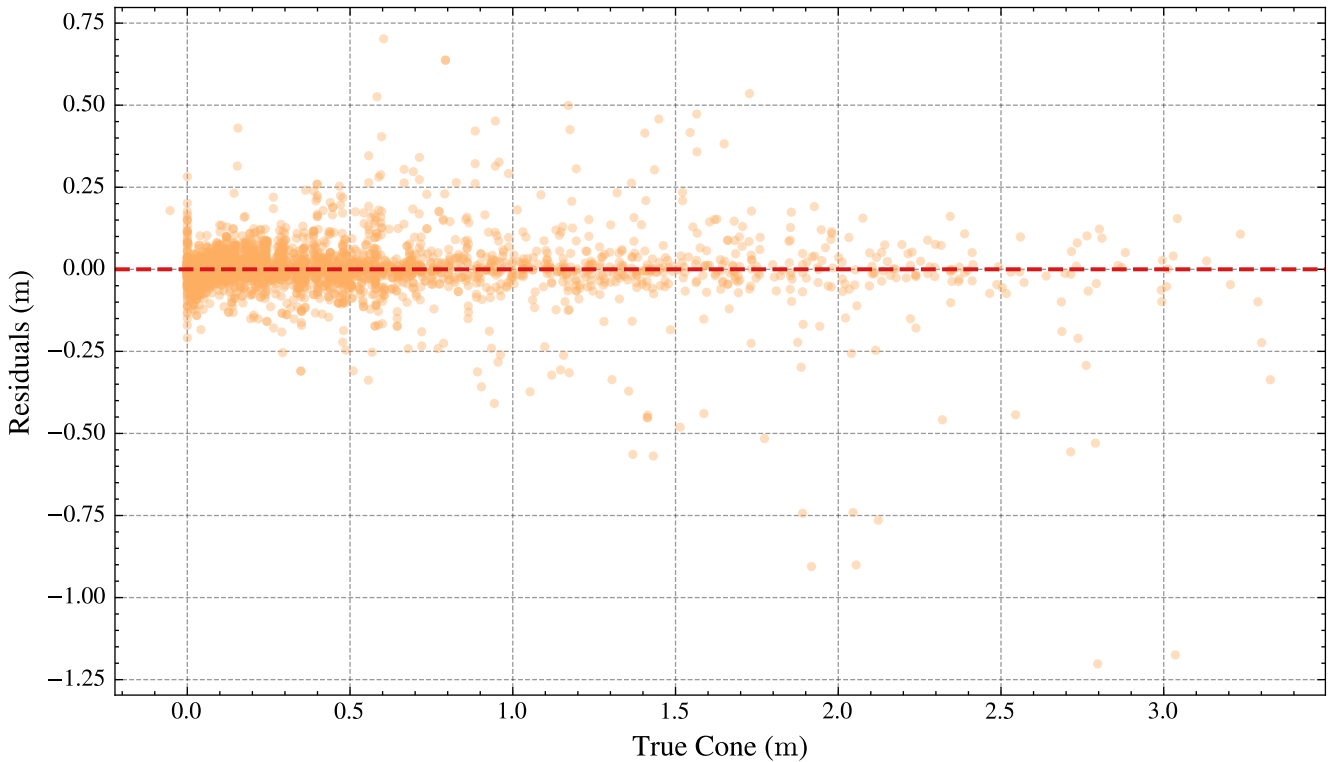
edRVFL-SC (Pareto winner) — Residuals for Cone
