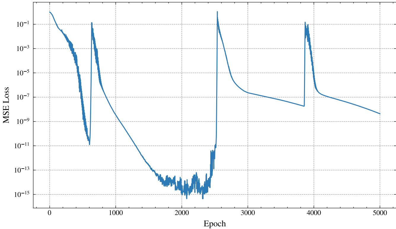
MLP Training Loss — Cone (10 samples)
