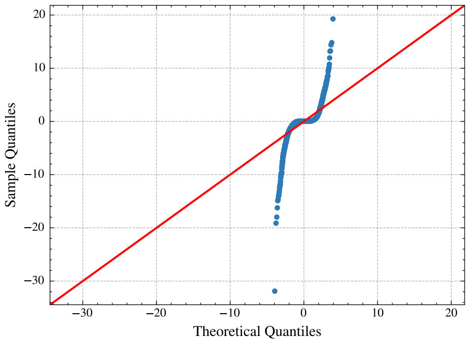
Q-Q Plot — Area
