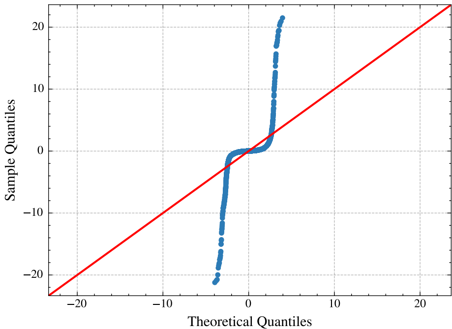
Q-Q Plot — Iso_distance
