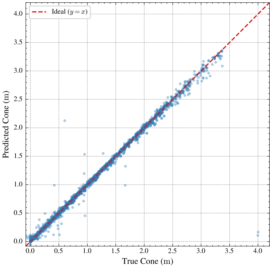
Optimized MLP — Cone R^2 = 0.9909 , RMSE = 0.05 m
