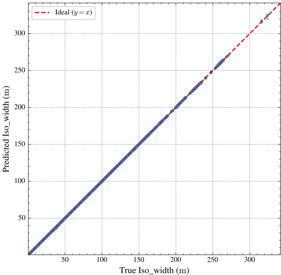
Optimized MLP — Iso_width R^2 = 1.0000 , RMSE = 0.07 m
