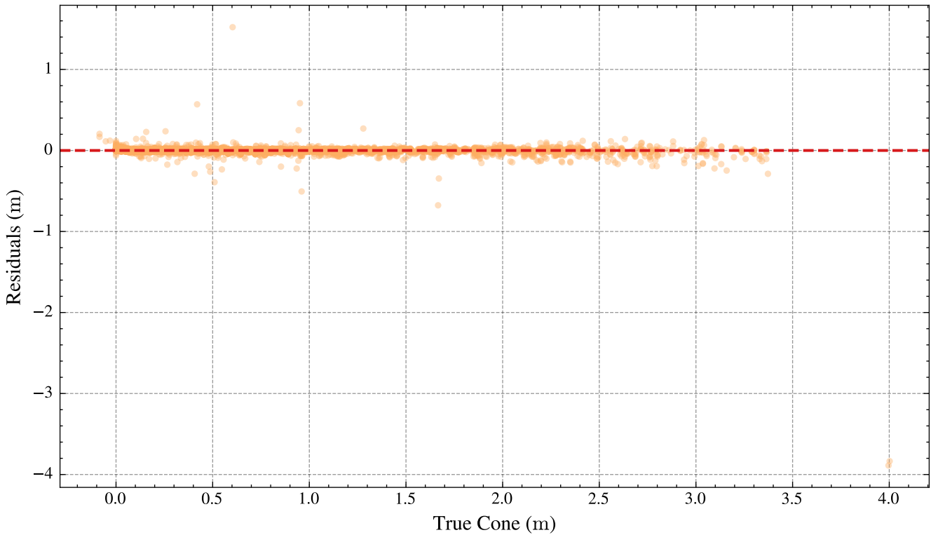
Optimized MLP — Residuals for Cone
